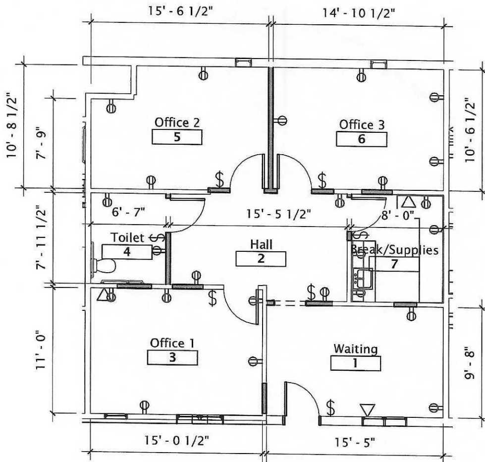
1 Dimension Plan 402B A2 1/8" = 1'-0"
